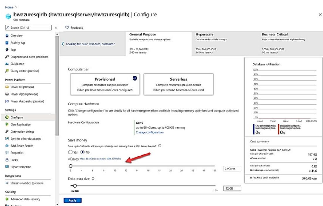
Figure 7-17. Using the Azure portal to increase vCores
