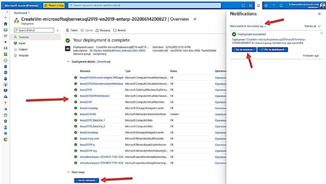
Figure 3-18. Deployment complete for SQL Server in Azure Virtual Machine
