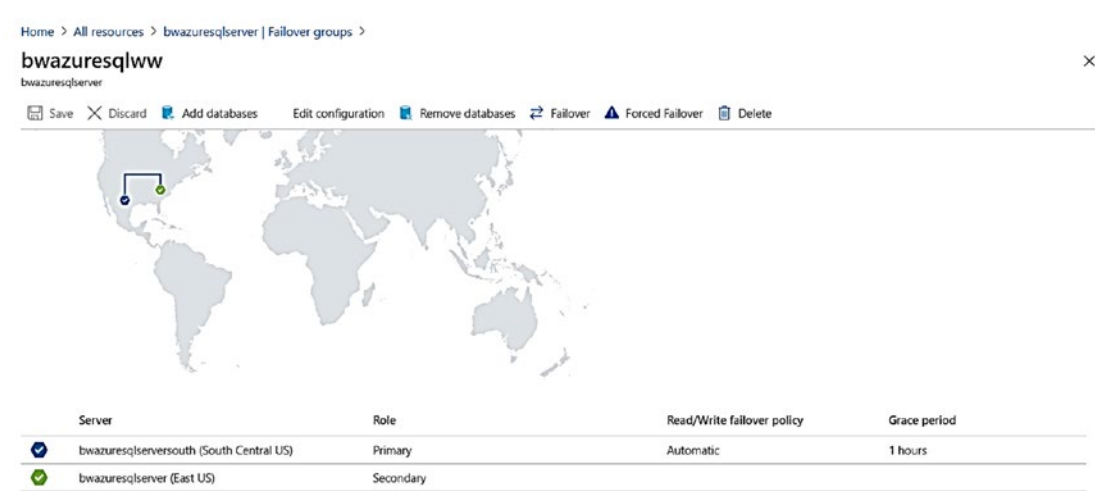
Figure 8-34. Failover group status after a failover
