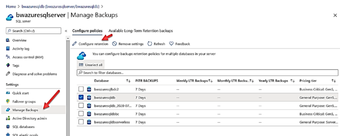
Figure 8-8. Configuring backup retention for Azure SQL Database
