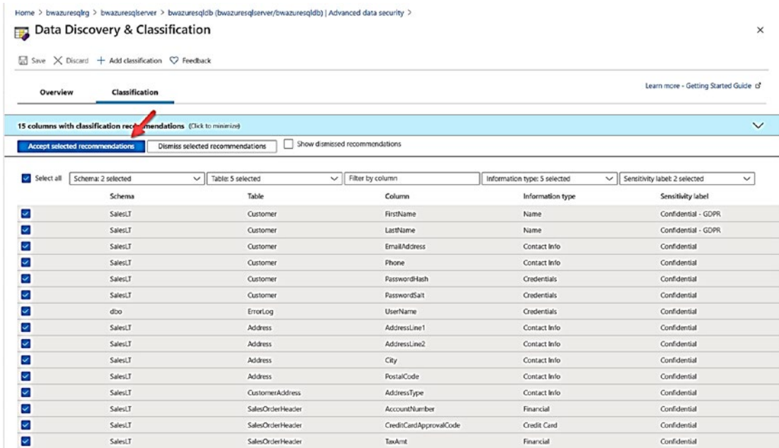
Figure 6-33. Recommendations for Data Classification
