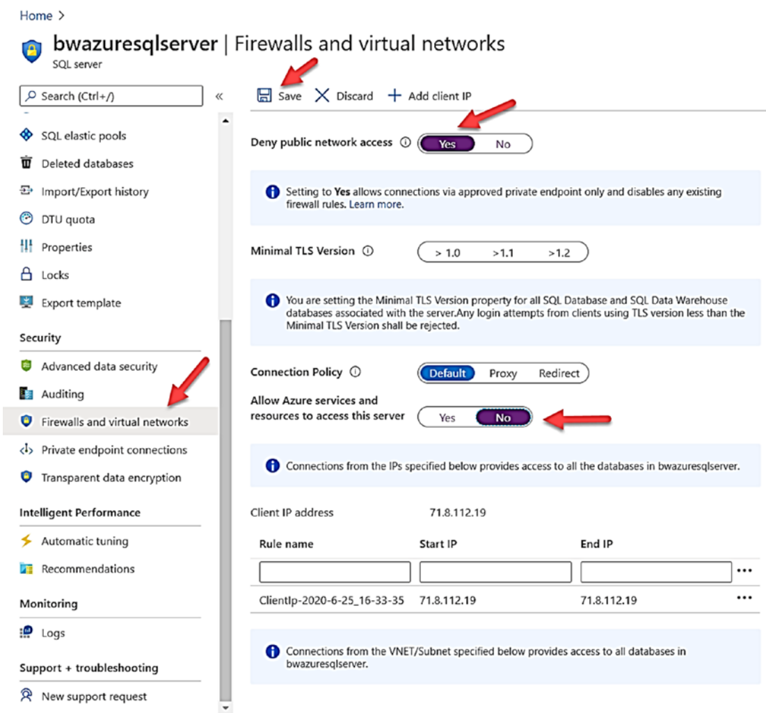
Figure 6-4. Turning off public endpoint for Azure SQL Database
