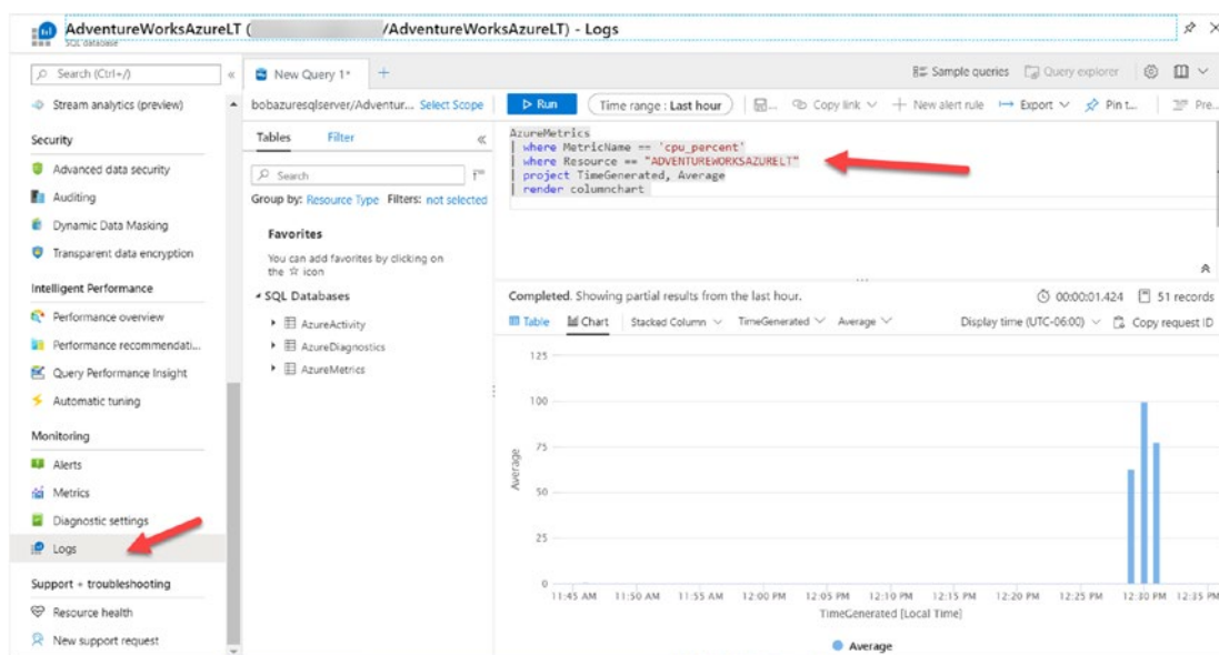
Figure 7-15. Using Kusto to view resource usage from Azure Monitor Logs
