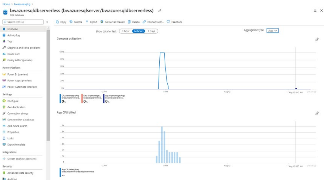
Figure 7-23. Serverless scale and compute billing
