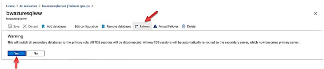
Figure 8-32. Failing over a failover group for Azure SQL Database
