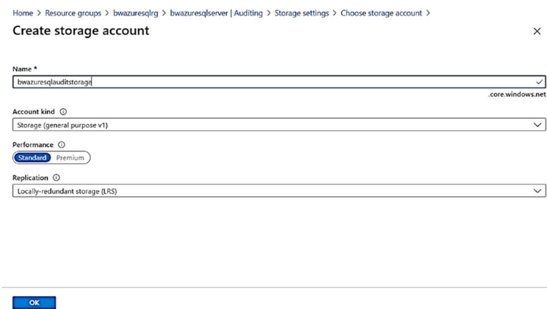
Figure 6-23. Creating a new storage account for auditing for Azure SQL Database
