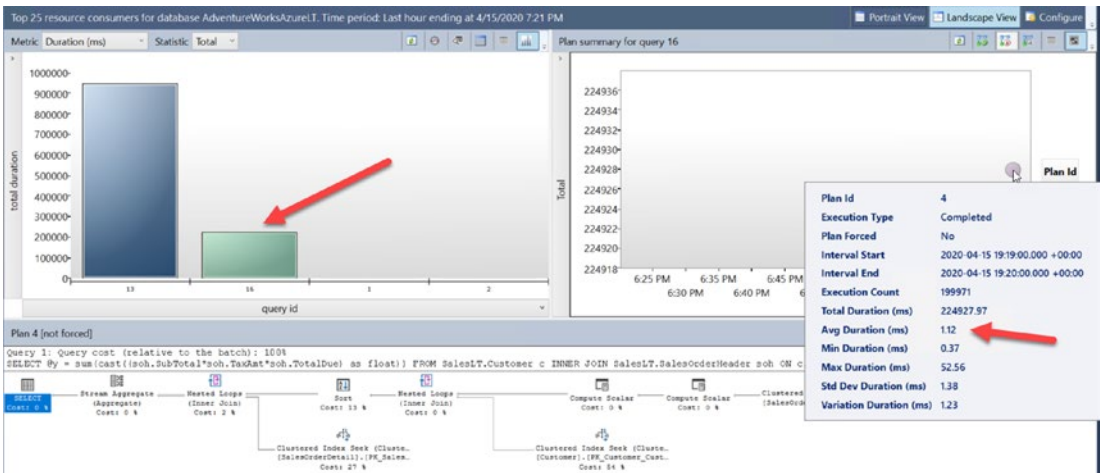
Figure 7-19. Top Consuming Query report with a faster query
