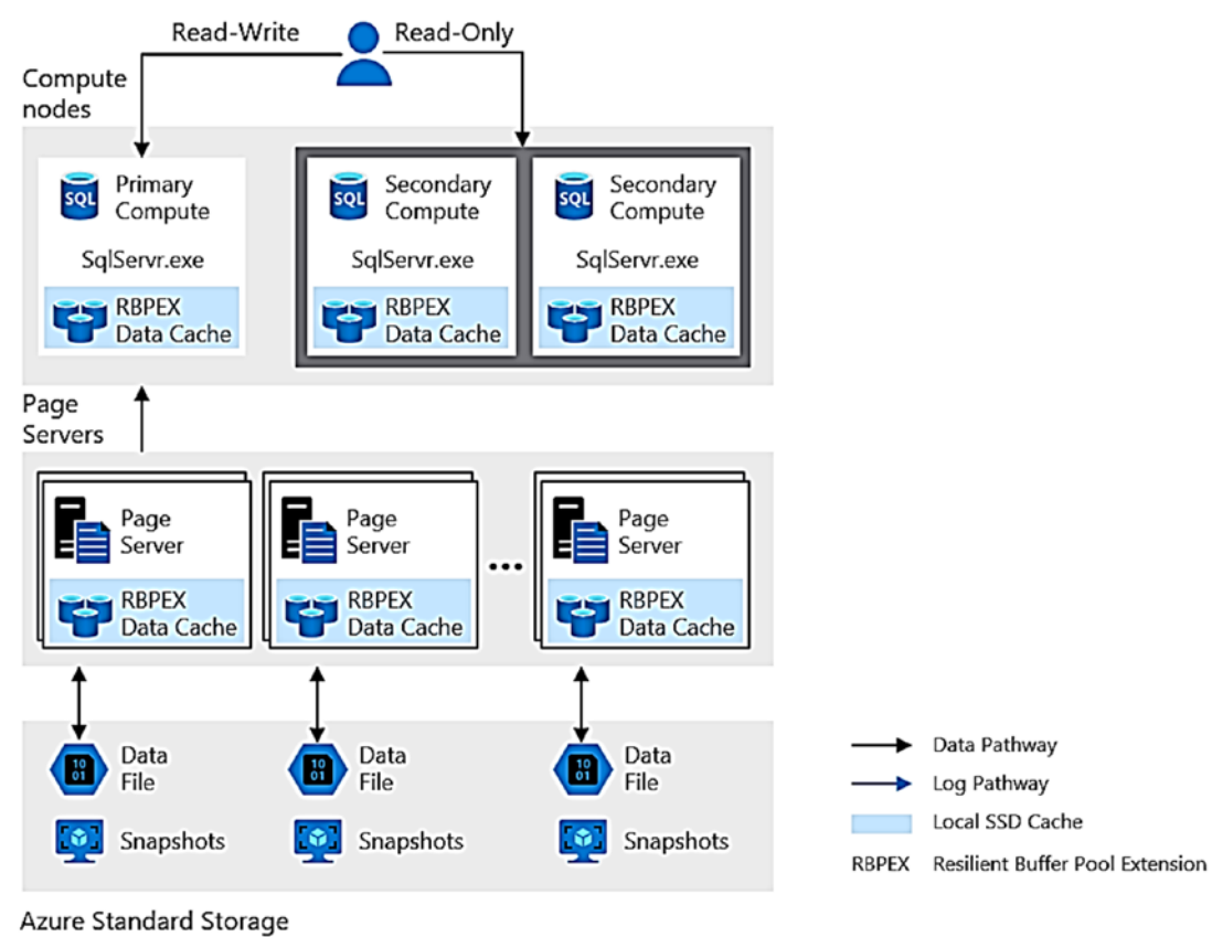
Figure 8-17. Data files for Hyperscale on Azure storage
