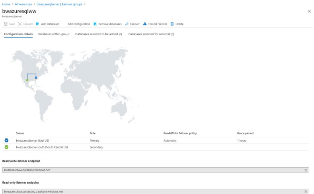
Figure 8-30. Configuration and managing a failover group in the Azure portal
