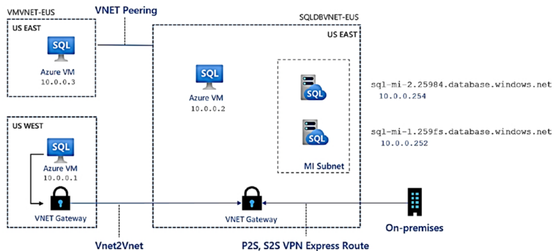
Figure 6-1. Network security to Azure SQL Managed Instance
