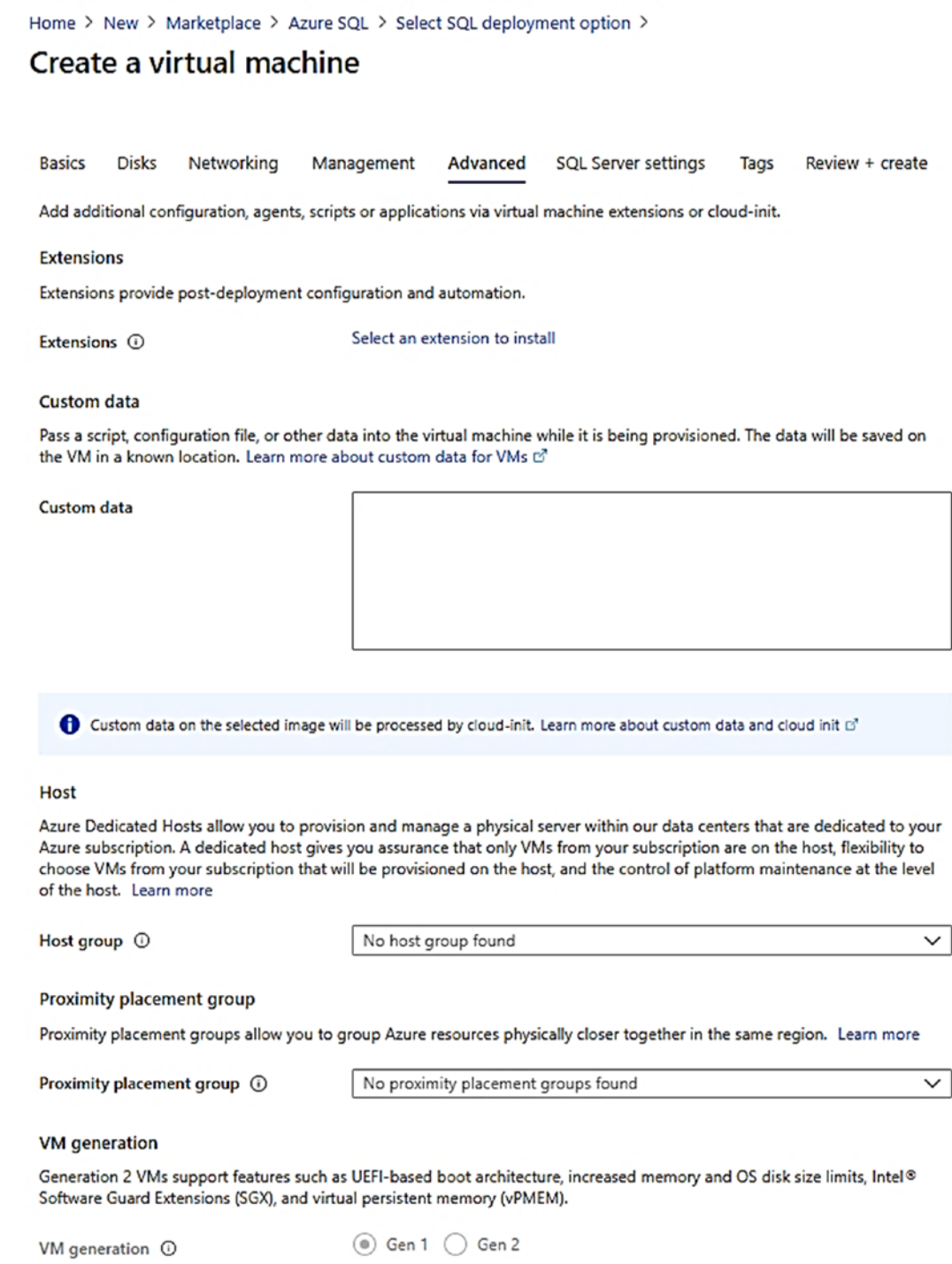
Figure 3-11. Advanced options for Azure VM
