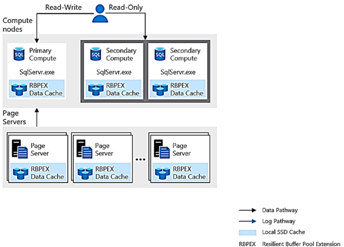
Figure 8-16. Page servers in a Hyperscale deployment
