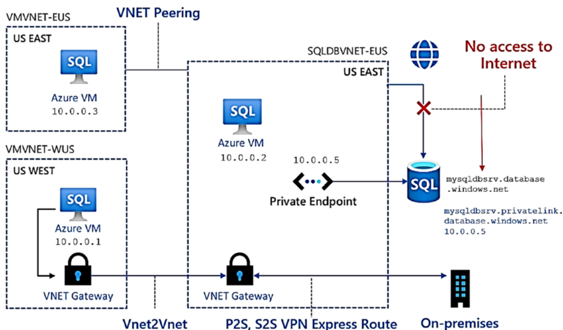
Figure 6-3. Private link with Azure SQL Database
