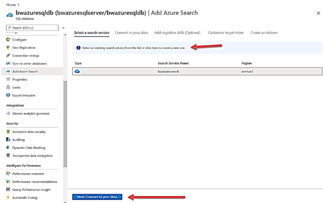
Figure 10-4. Connect Azure search with Azure SQL Database
