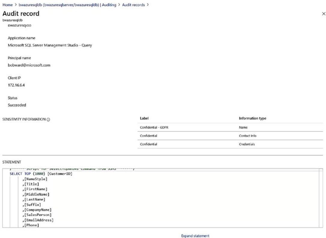
Figure 6-36. An audit record showing sensitivity information access
