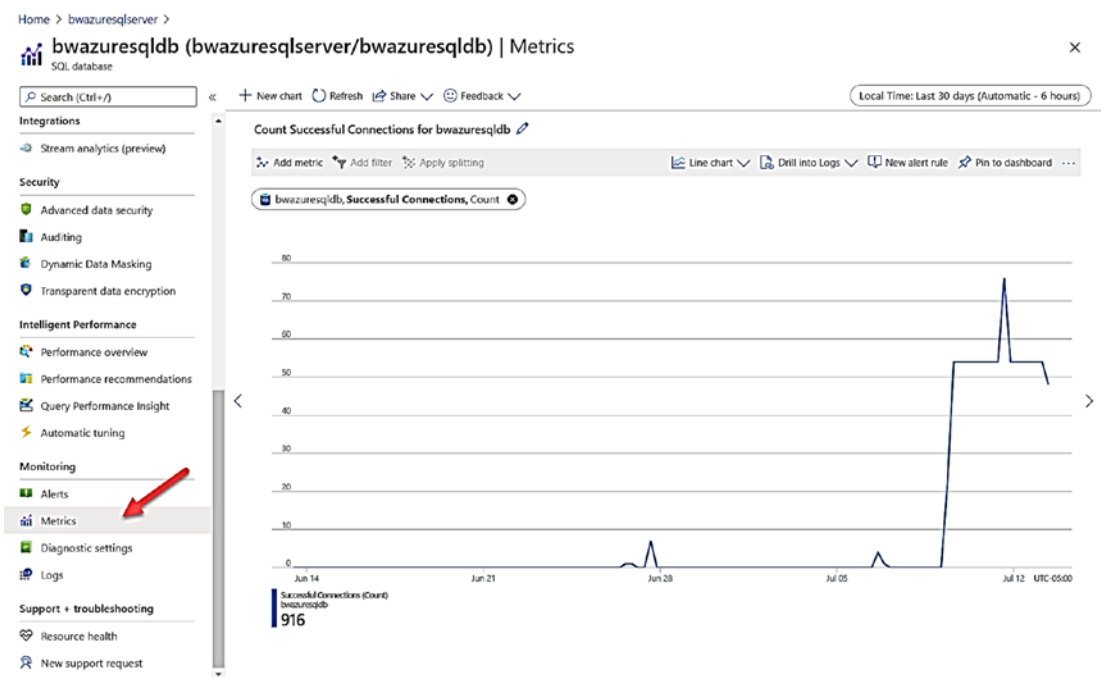
Figure 6-20. Tracking successful connections with Azure Metrics
