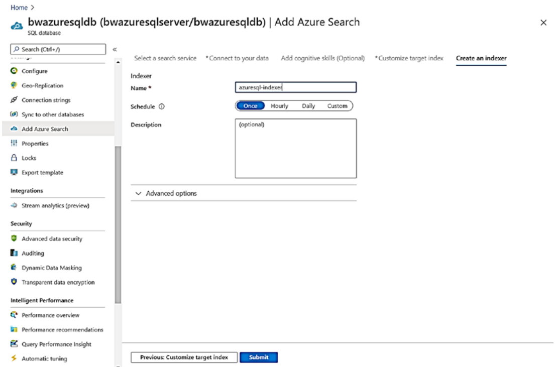
Figure 10-7. Creating an indexer for Azure Search
