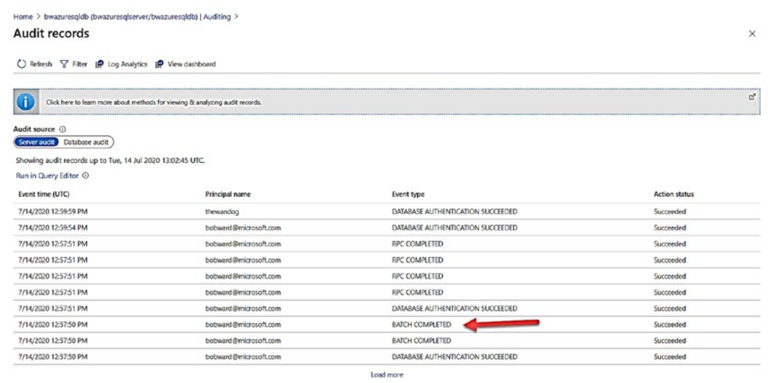
Figure 6-35. Audit records from SQL Database Audit
