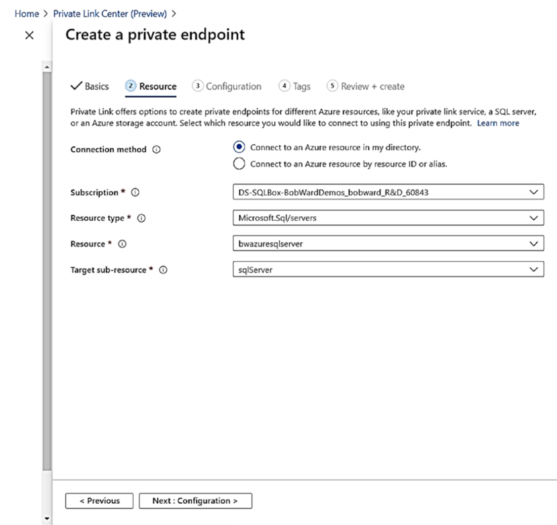
Figure 6-8. Associating the private endpoint with Azure SQL Database
