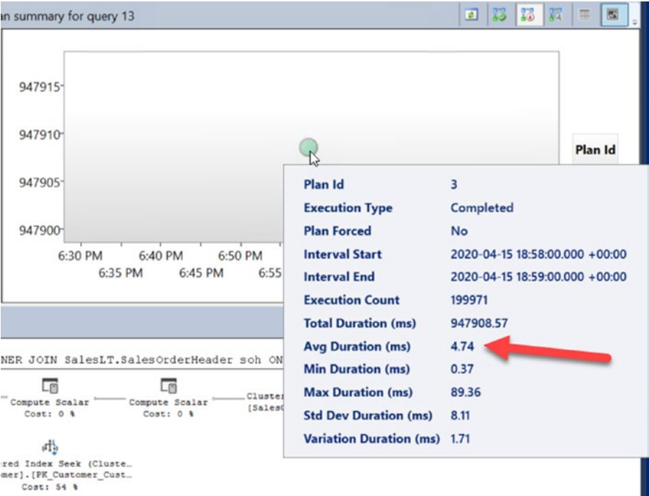
Figure 7-9. Query stats for a query plan
