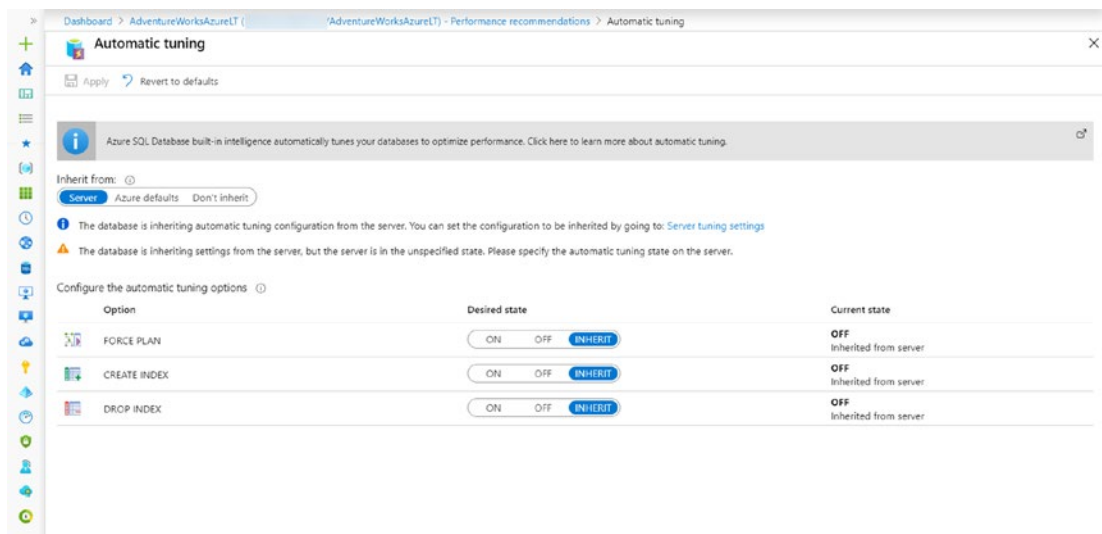
Figure 7-28. Setting automatic tuning options
