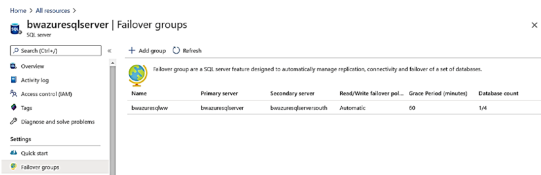
Figure 8-29. Failover group after deployment
