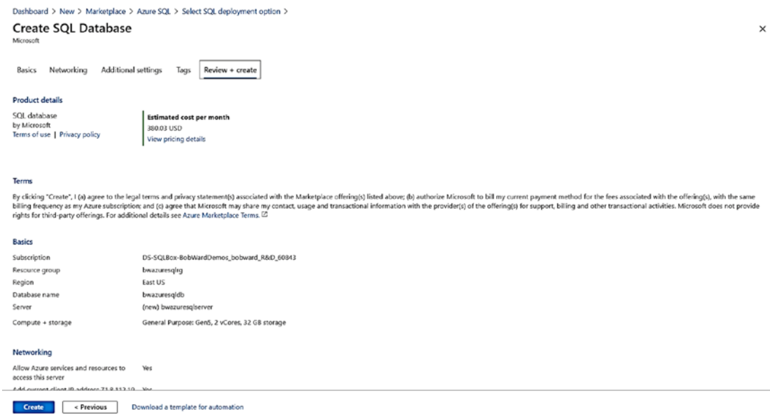
Figure 4-20. Final screen before deployment of Azure SQL Database
