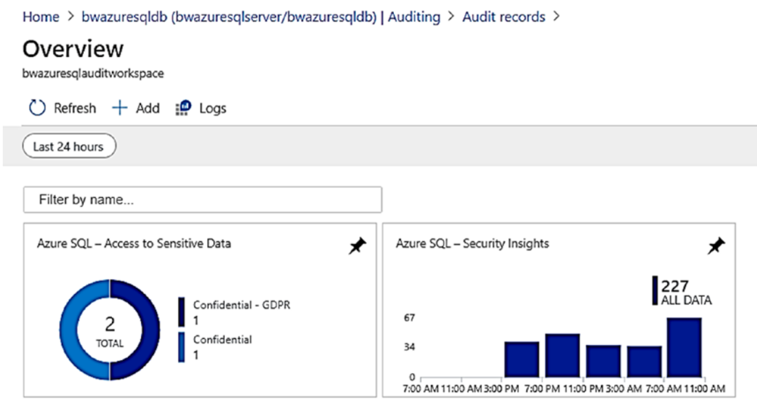
Figure 6-37. Log analytics dashboard showing access to sensitive data
