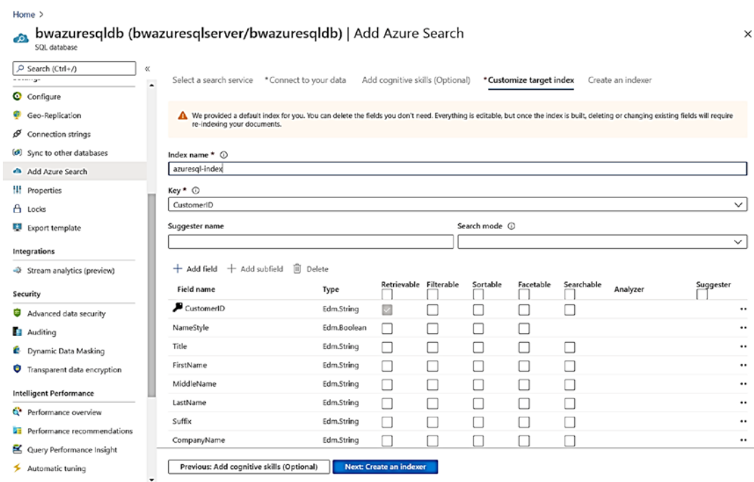
Figure 10-6. Customizing the search index
