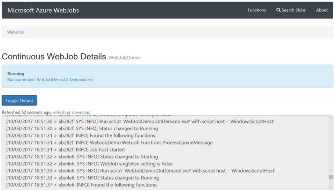
Figure 8-20. The Azure dashboard. For continuous WebJobs, we can see the function that is running, how long it's been running, and Toggle Output to view logs. These logs are useful as a starting point for troubleshooting issues in deployment.
