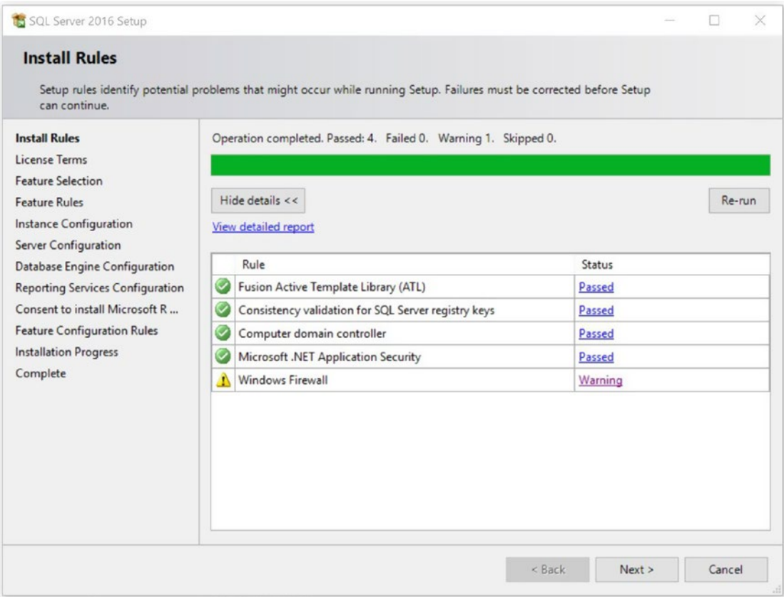
Figure 1-3. The rule check will ensure that your system has everything needed for SQL Server. Click the hyperlink in the Status column to see a description of the problem if any rule fails or raises a warning.
