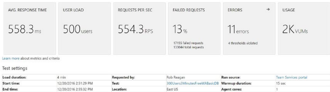
Figure 2-15. Results for our second load test that caused errors
