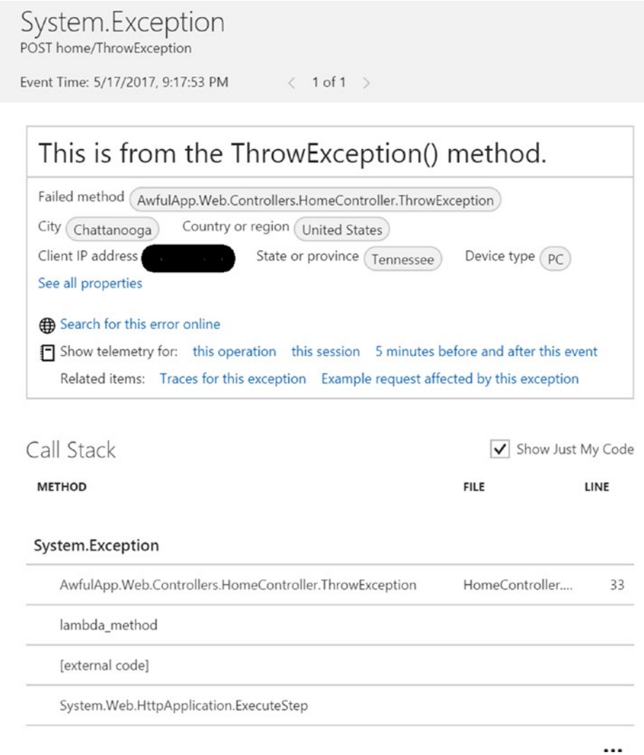
Figure 11-19. Application Insights provides a great deal of information on exceptions
