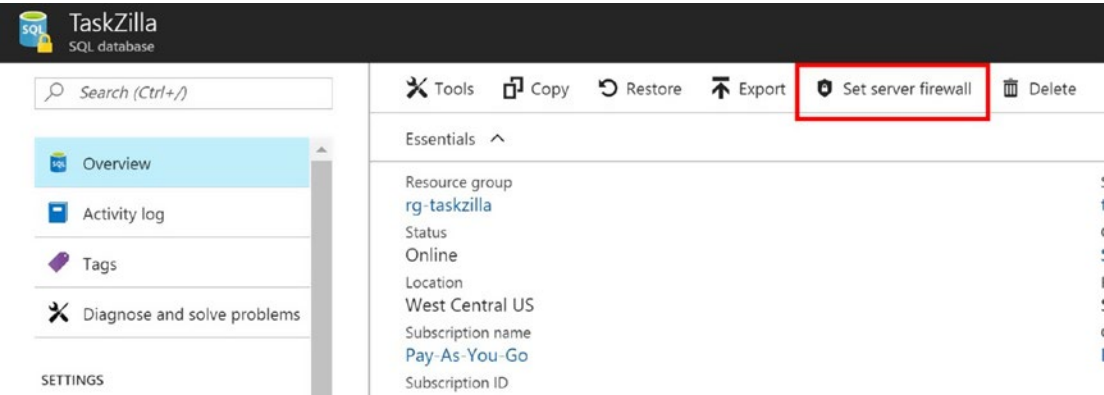
Figure 4-13. The SQL Database Overview blade has a link to set server firewall rules
